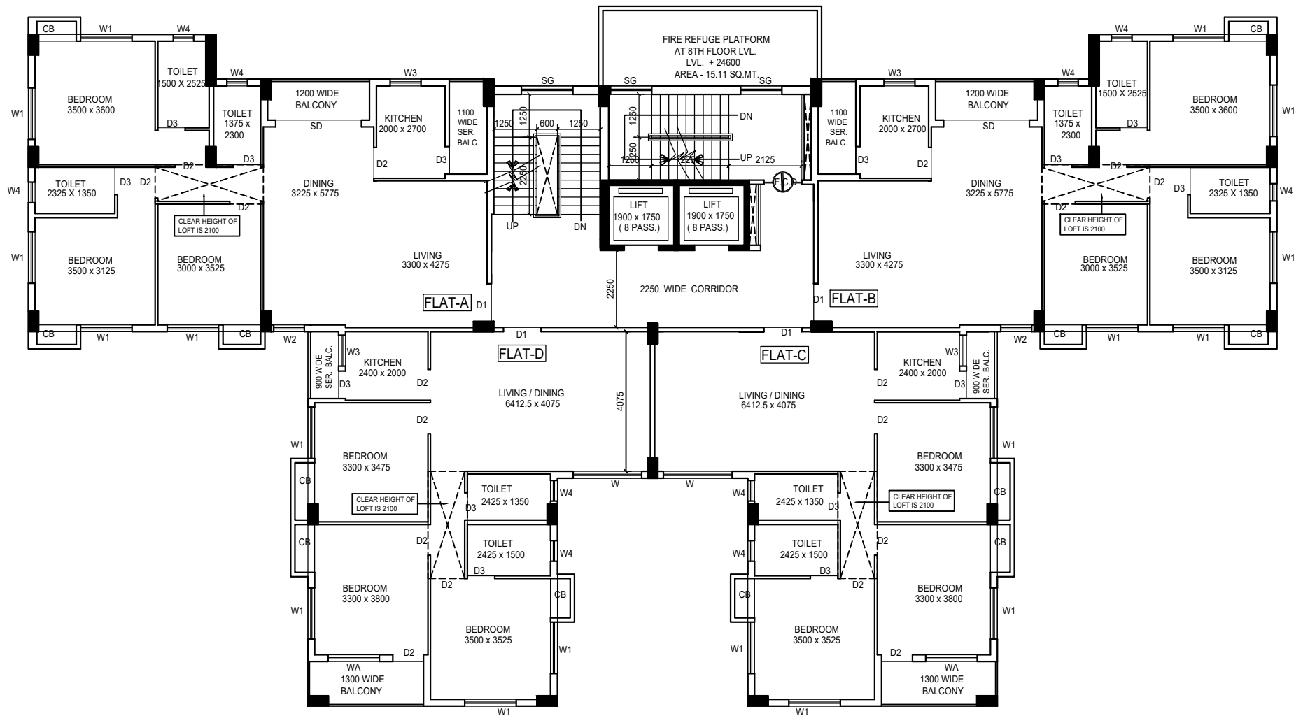
HIG BUILDING (BLOCK- I)
